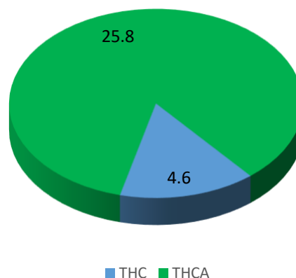
Cannabinoids Profile
