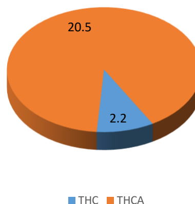
Cannabinoids Profile
